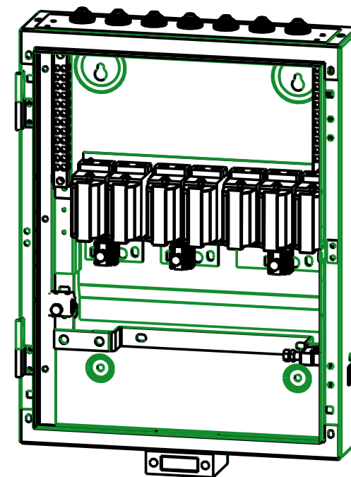
ISOMETRIC VIEW WITH DOOR AND CABLE SCREEN REMOVED
