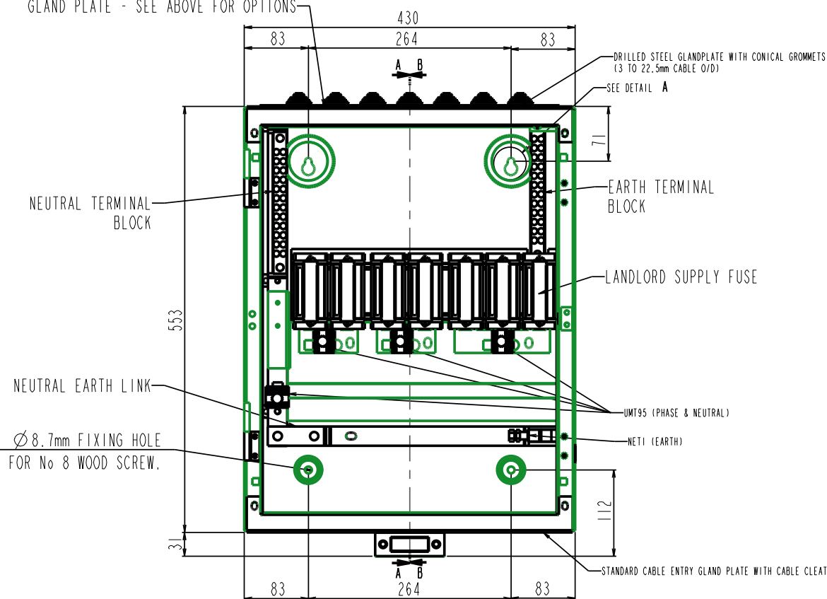
FRONT VIEW WITH DOOR AND CABLE SCREEN REMOVED
